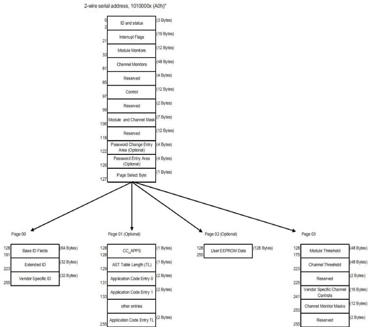
Figure 4, QSFP+ Memory Map (Specific Data Field Descriptions)
