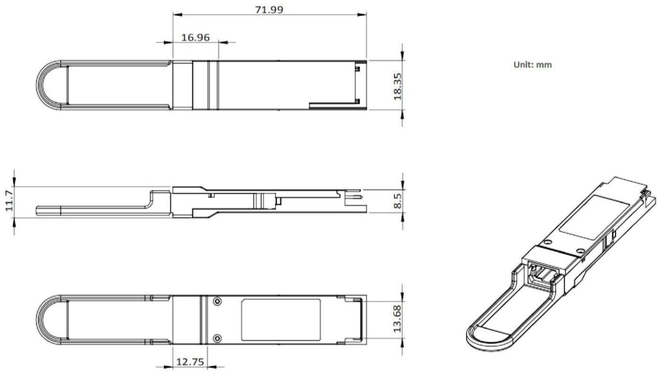
Figure 7, Mechanical Dimensions
