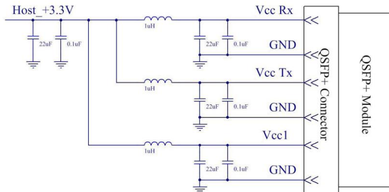
Figure 5, Recommended Host Board Power Supply Circuit
