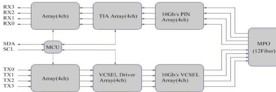
Figure 1. Transceiver functional Block Diagram
